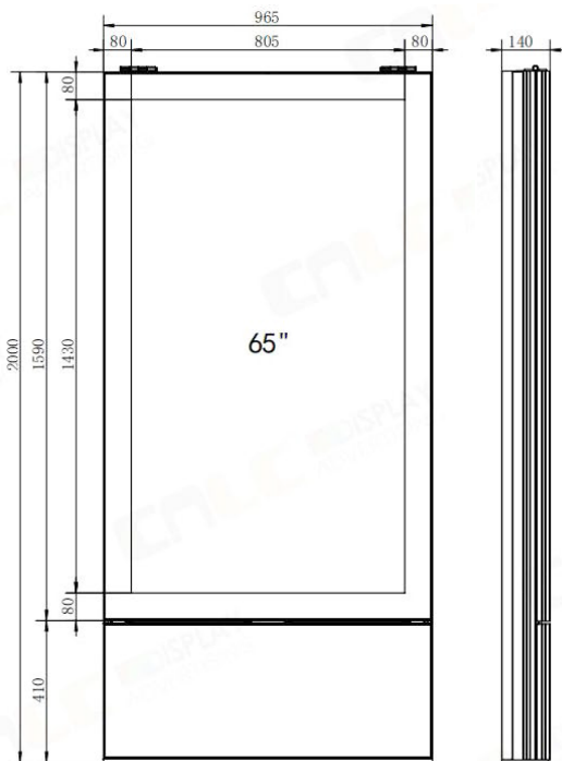
IDS65S1, ITK65S1 - 65" Single-sided
