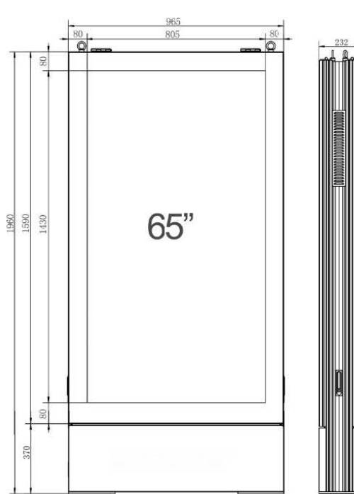
IDS65S2, ITK65S2 - 65" Double-sided
