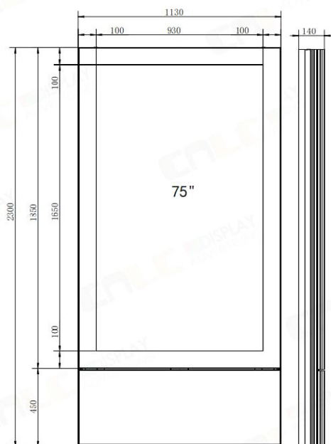
IDS75S1, ITK75S1 - 75" Single-sided
