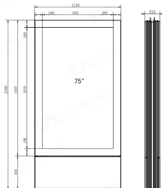
IDS75S2, ITK75S2 - 75" Double-sided
